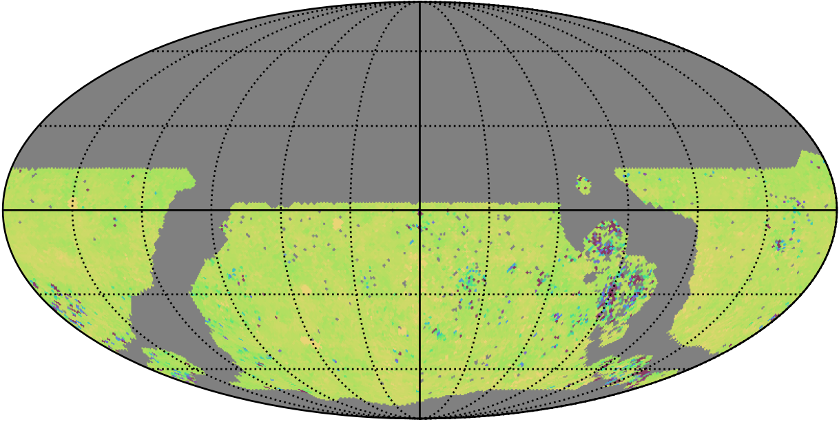
roll_pause_mjdp60_v3.4_10yrs WFD ug bands: 75th Percentile Intranight Timespan
