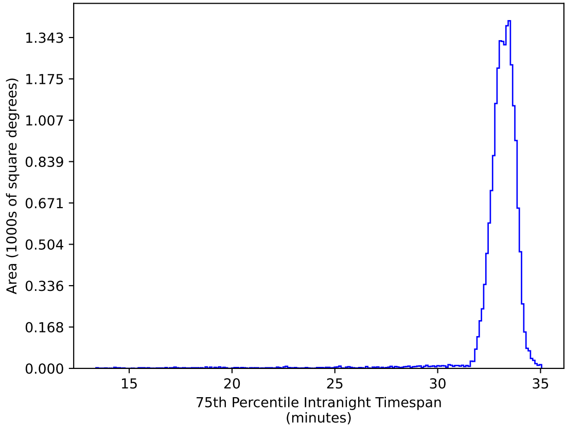
roll_pause_mjdp60_v3.4_10yrs WFD ug bands: 75th Percentile Intranight Timespan
