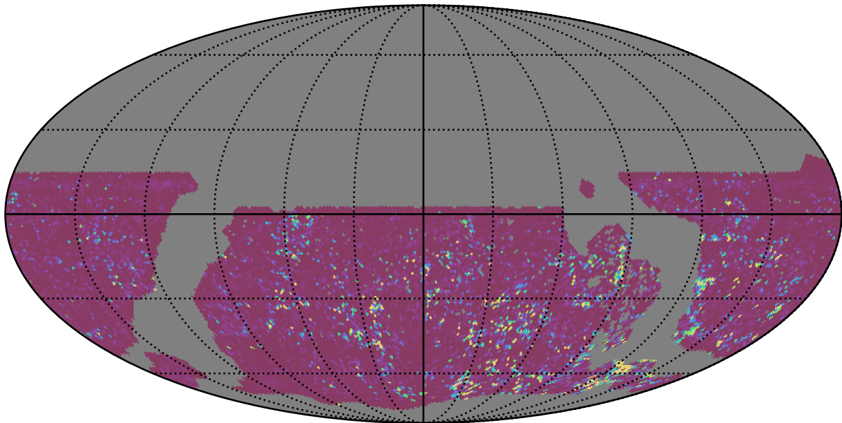
roll_pause_mjdp60_v3.4_10yrs WFD u band: 75th Percentile Intranight Timespan
