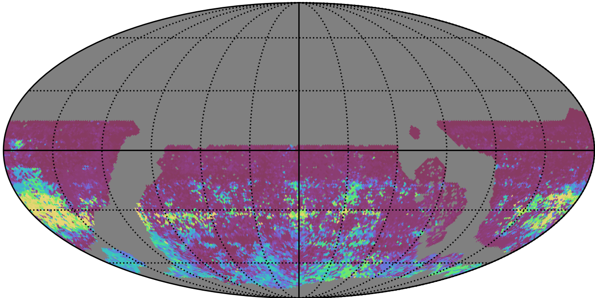
roll_pause_mjdp60_v3.4_10yrs WFD r band: 75th Percentile Intranight Timespan
