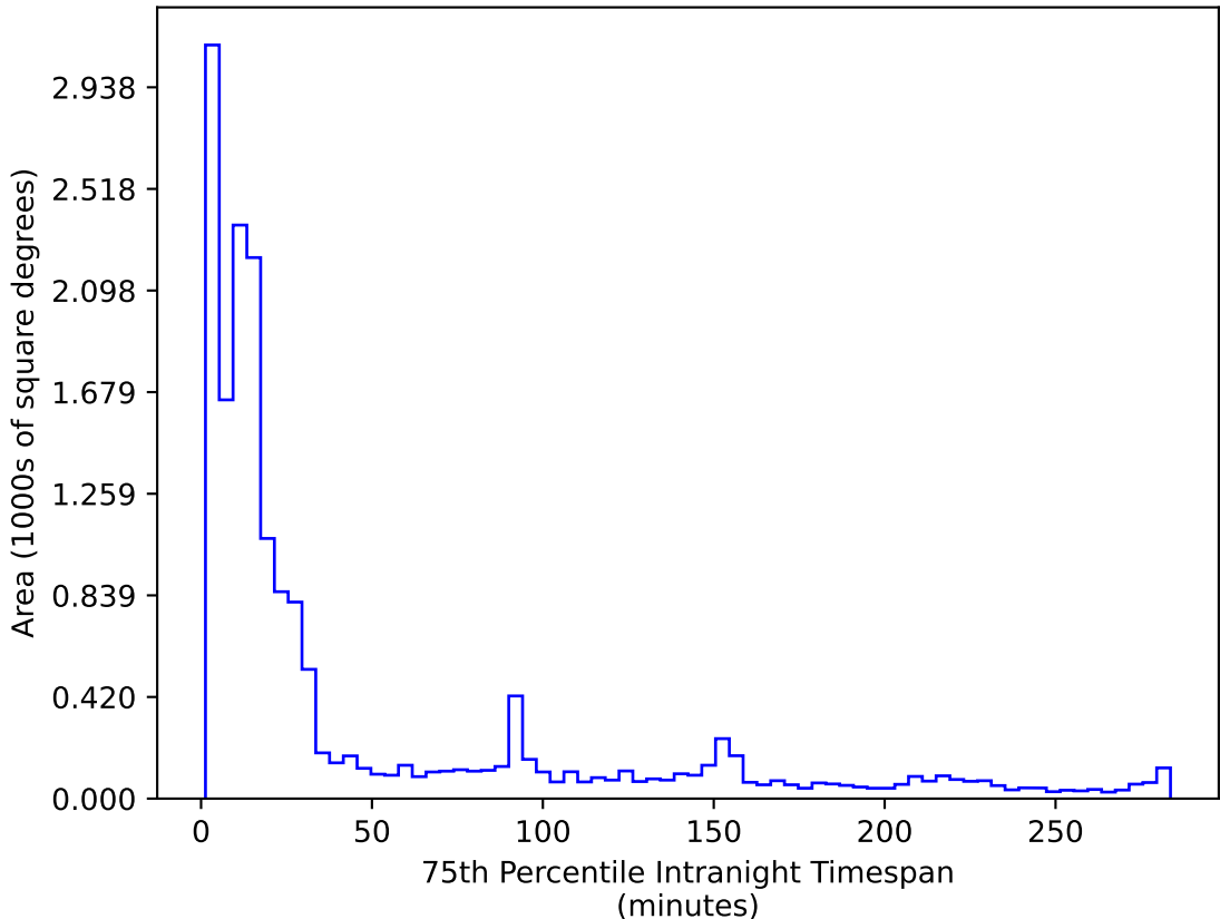
roll_pause_mjdp60_v3.4_10yrs WFD r band: 75th Percentile Intranight Timespan
