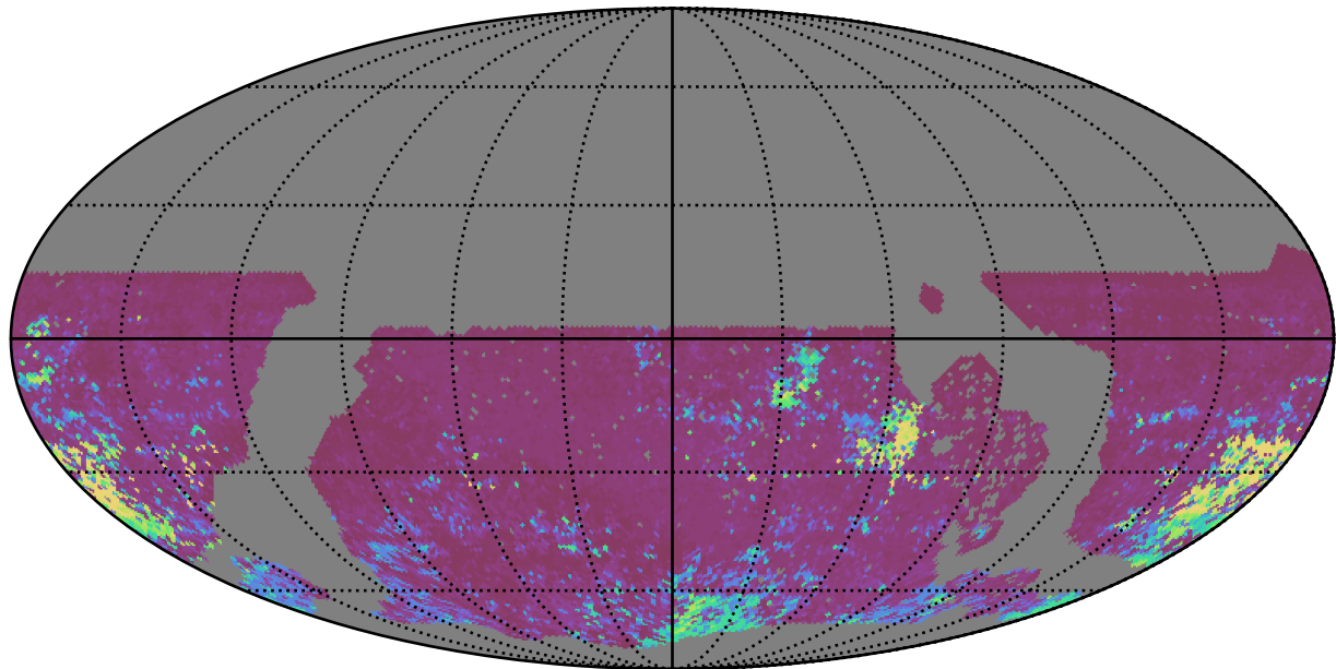
roll_pause_mjdp60_v3.4_10yrs WFD i band: 75th Percentile Intranight Timespan
