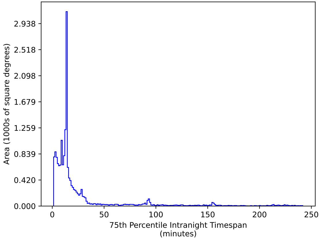
roll_pause_mjdp60_v3.4_10yrs WFD i band: 75th Percentile Intranight Timespan
