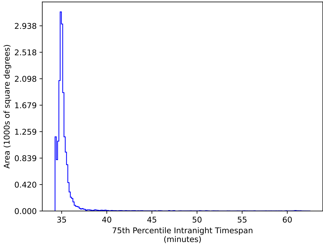
roll_pause_mjdp60_v3.4_10yrs WFD gr bands: 75th Percentile Intranight Timespan
