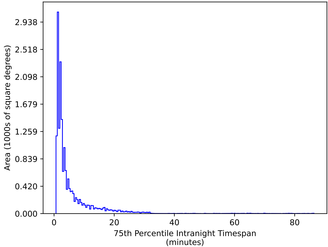
roll_pause_mjdp60_v3.4_10yrs WFD g band: 75th Percentile Intranight Timespan
