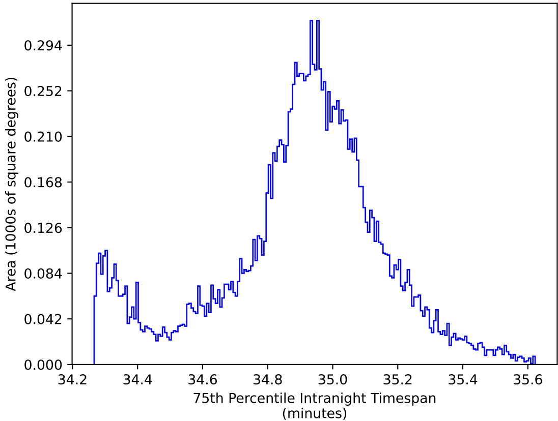
roll_pause_mjdp60_v3.4_10yrs WFD all bands: 75th Percentile Intranight Timespan
