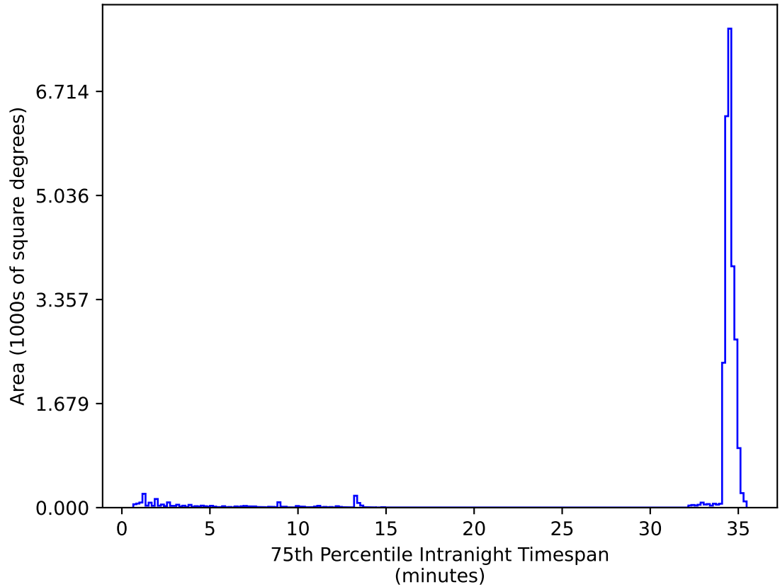
roll_pause_mjdp60_v3.4_10yrs All sky zy bands: 75th Percentile Intranight Timespan
