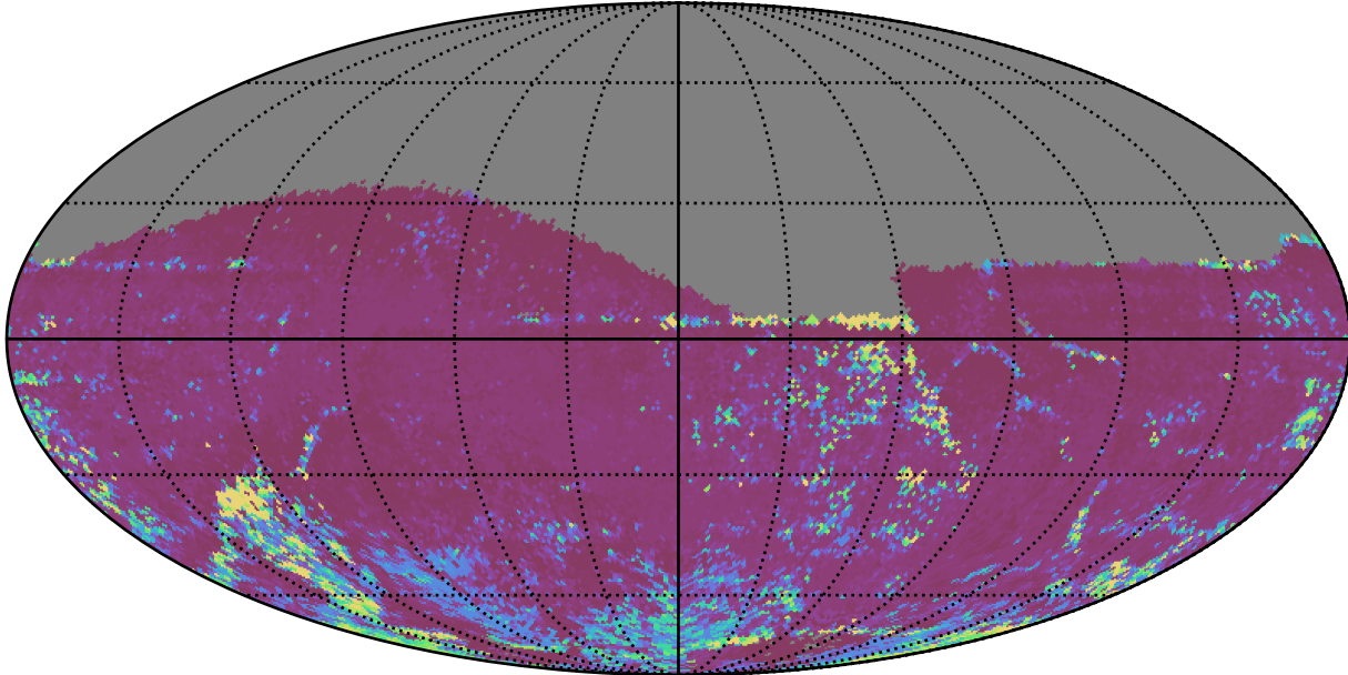
roll_pause_mjdp60_v3.4_10yrs All sky z band: 75th Percentile Intranight Timespan
