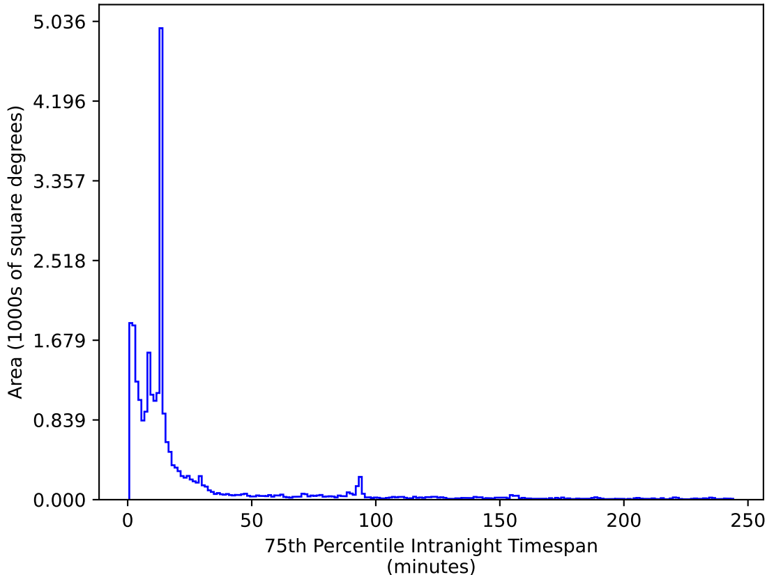
roll_pause_mjdp60_v3.4_10yrs All sky z band: 75th Percentile Intranight Timespan
