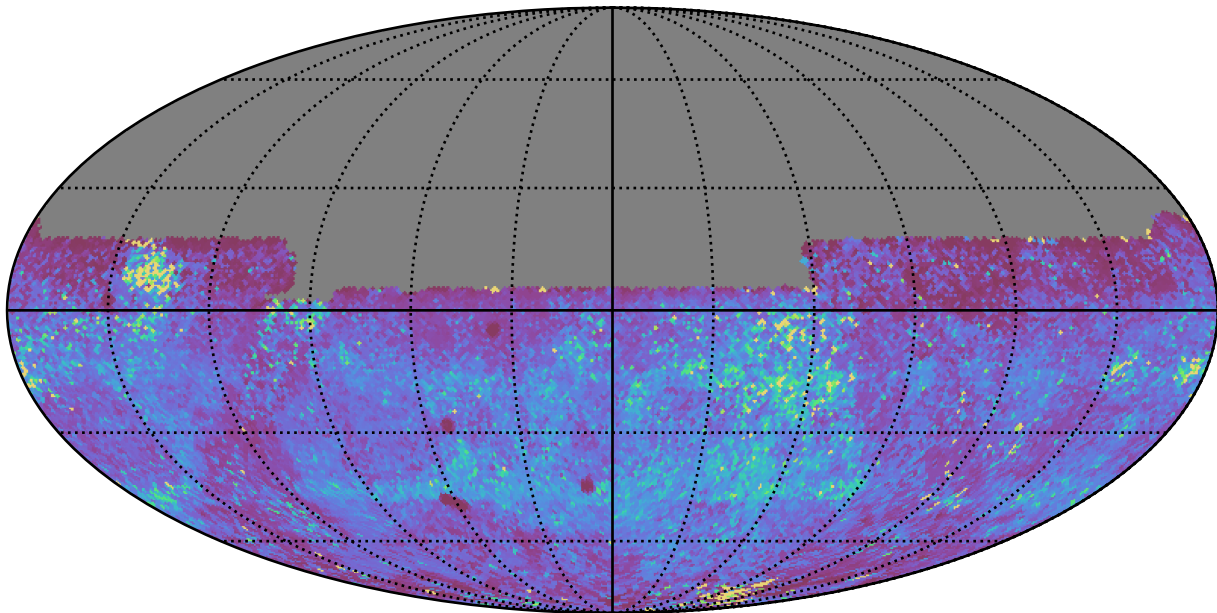
roll_pause_mjdp60_v3.4_10yrs All sky y band: 75th Percentile Intranight Timespan
