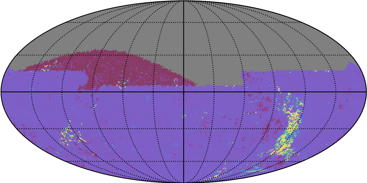
roll_pause_mjdp60_v3.4_10yrs All sky ug bands: 75th Percentile Intranight Timespan
