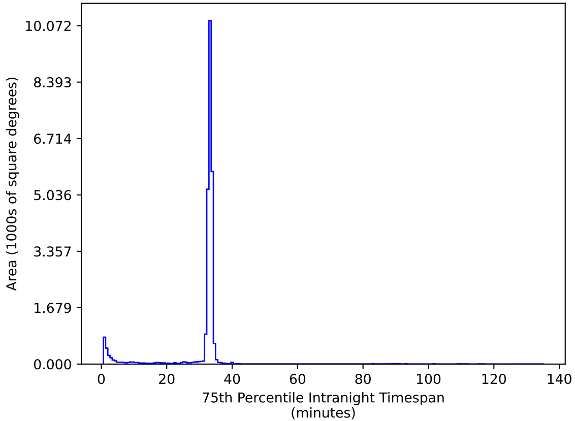
roll_pause_mjdp60_v3.4_10yrs All sky ug bands: 75th Percentile Intranight Timespan
