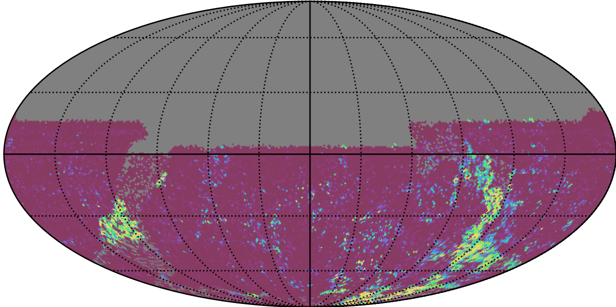
roll_pause_mjdp60_v3.4_10yrs All sky u band: 75th Percentile Intranight Timespan
