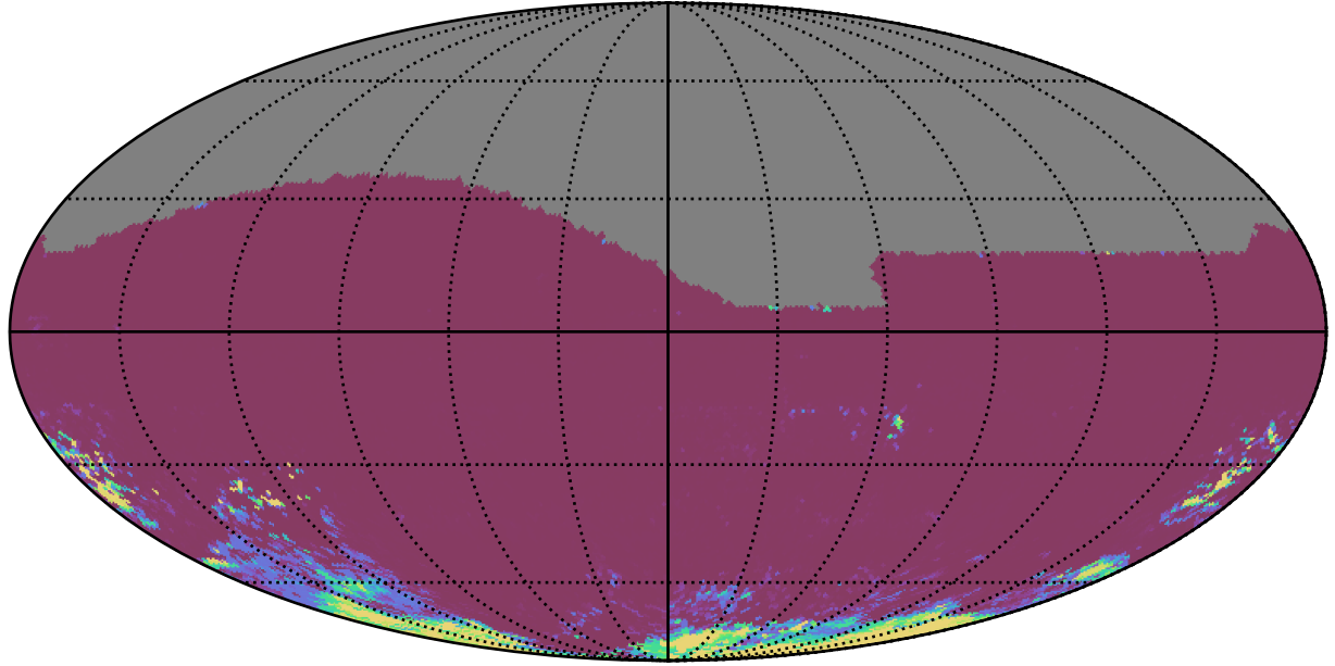
roll_pause_mjdp60_v3.4_10yrs All sky ri bands: 75th Percentile Intranight Timespan
