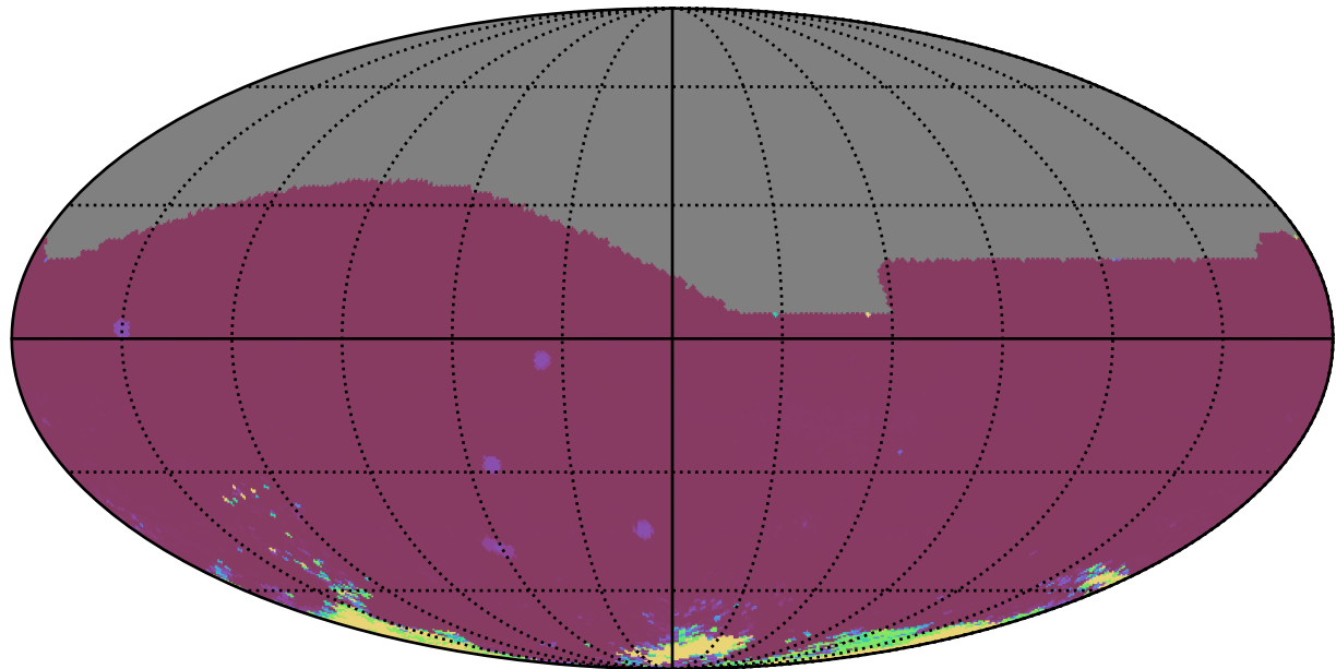
roll_pause_mjdp60_v3.4_10yrs All sky iz bands: 75th Percentile Intranight Timespan
