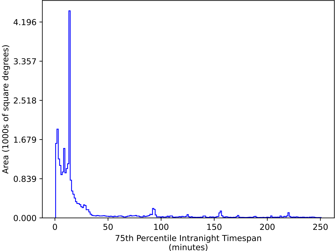
roll_pause_mjdp60_v3.4_10yrs All sky i band: 75th Percentile Intranight Timespan
