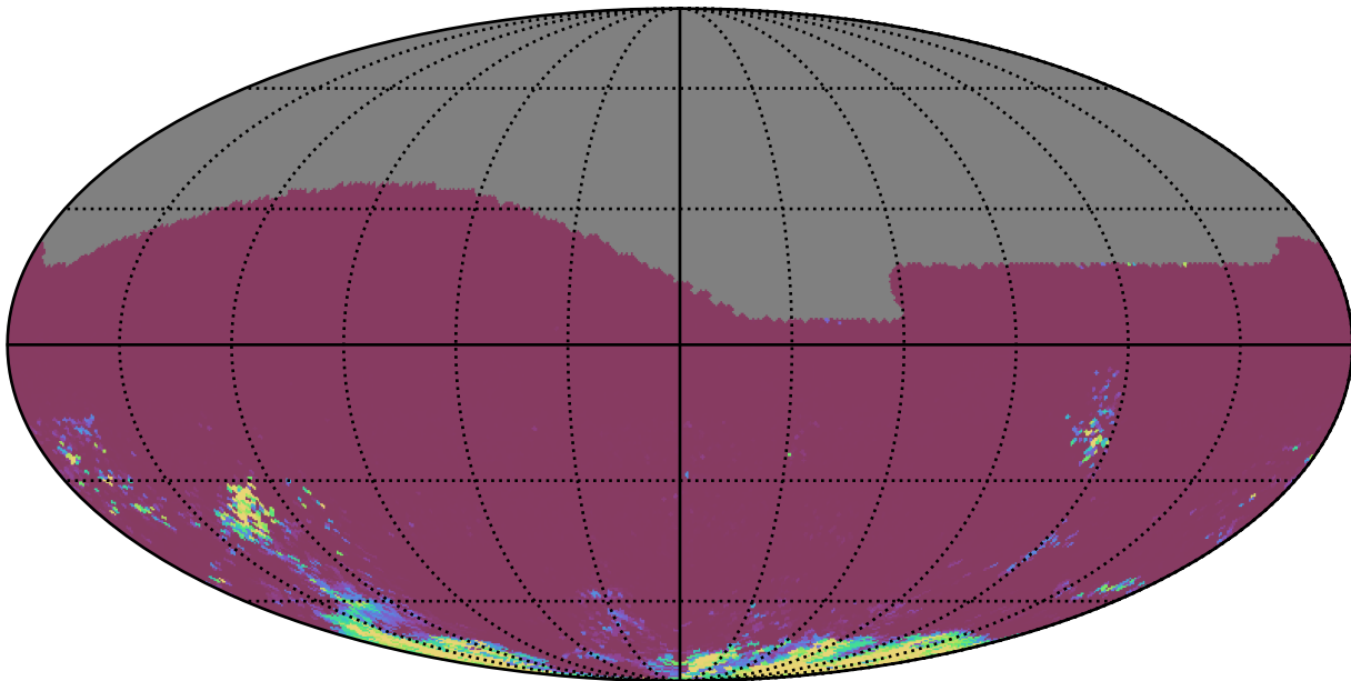
roll_pause_mjdp60_v3.4_10yrs All sky gr bands: 75th Percentile Intranight Timespan
