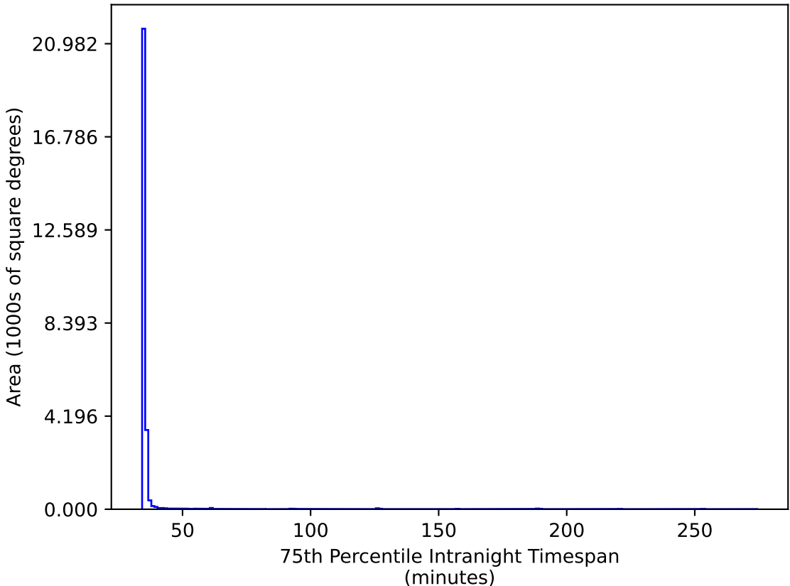
roll_pause_mjdp60_v3.4_10yrs All sky gr bands: 75th Percentile Intranight Timespan
