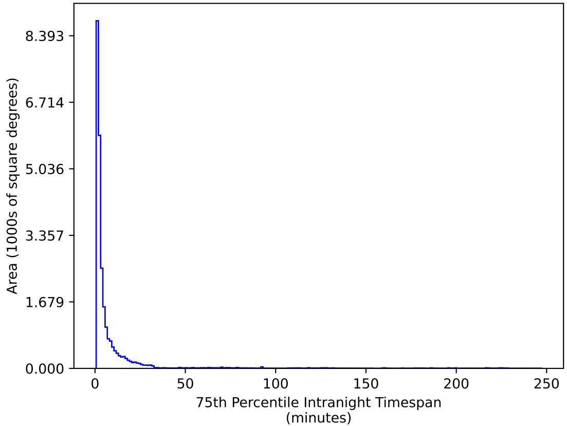
roll_pause_mjdp60_v3.4_10yrs All sky g band: 75th Percentile Intranight Timespan
