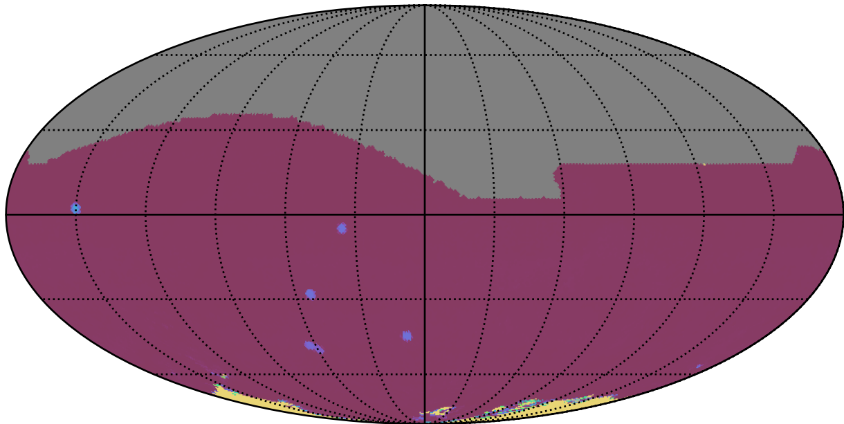
roll_pause_mjdp60_v3.4_10yrs All sky all bands: 75th Percentile Intranight Timespan
