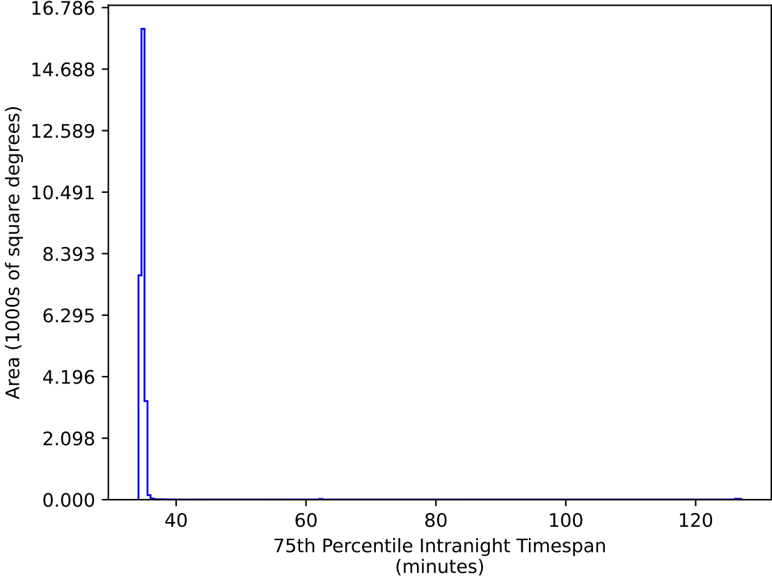
roll_pause_mjdp60_v3.4_10yrs All sky: 75th Percentile Intranight Timespan
