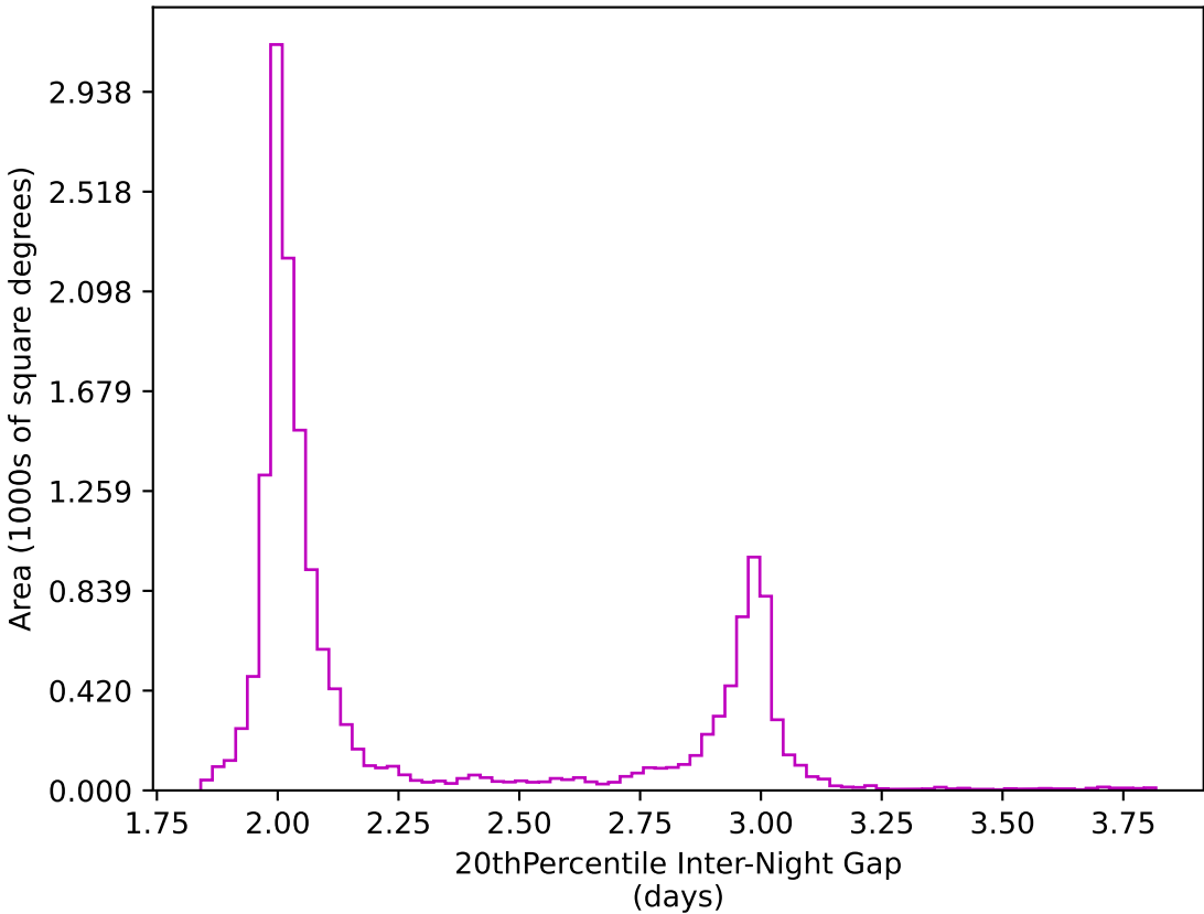
roll_pause_mjdp60_v3.4_10yrs WFD z band: 20thPercentile Inter-Night Gap
