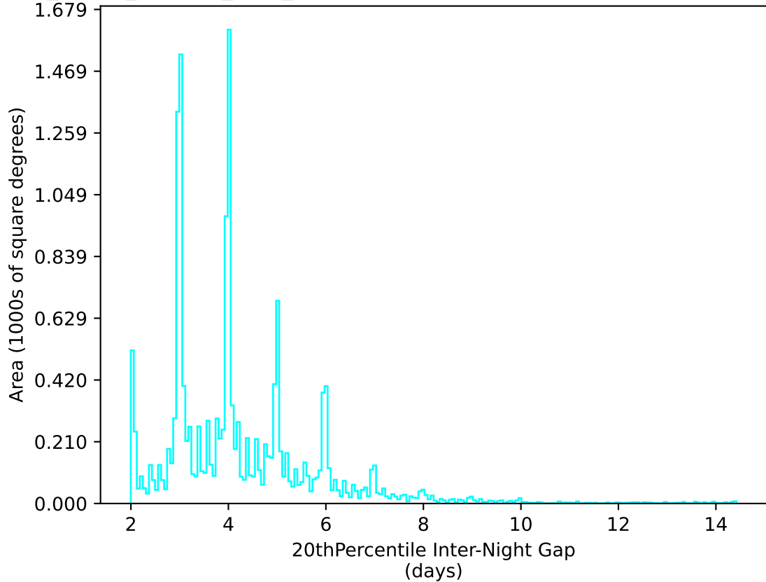
roll_pause_mjdp60_v3.4_10yrs WFD u band: 20thPercentile Inter-Night Gap
