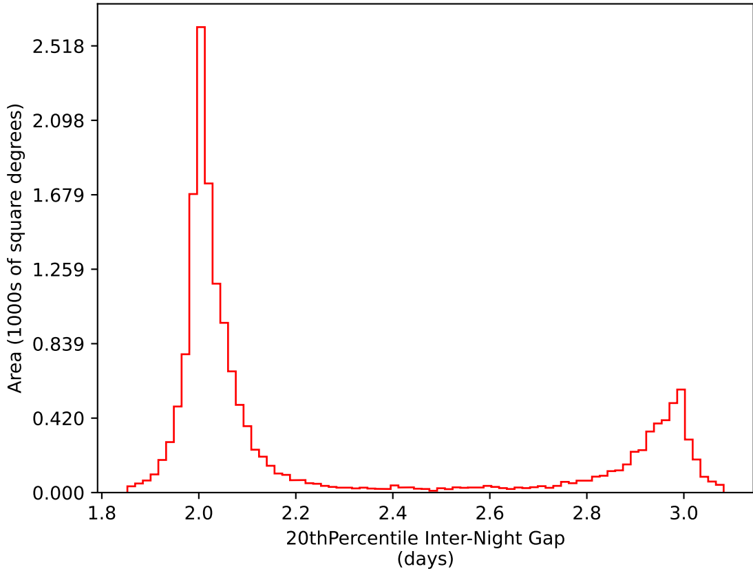
roll_pause_mjdp60_v3.4_10yrs WFD i band: 20thPercentile Inter-Night Gap
