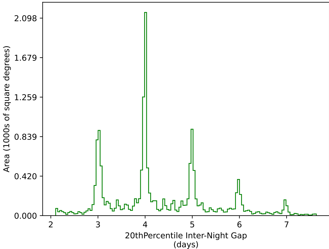
roll_pause_mjdp60_v3.4_10yrs WFD g band: 20thPercentile Inter-Night Gap
