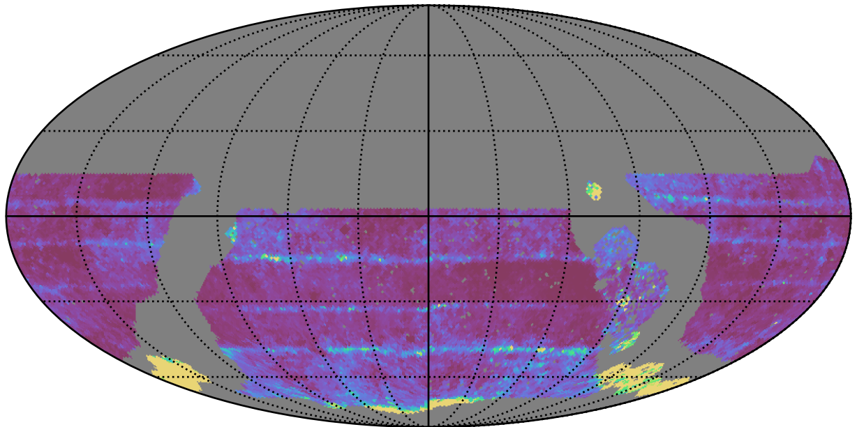
roll_pause_mjdp60_v3.4_10yrs WFD all bands: 20thPercentile Inter-Night Gap
