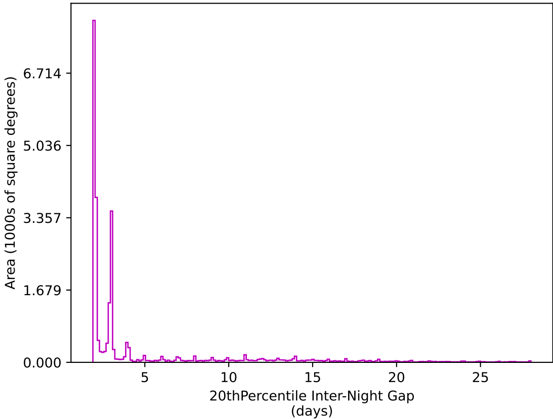
roll_pause_mjdp60_v3.4_10yrs All sky z band: 20thPercentile Inter-Night Gap
