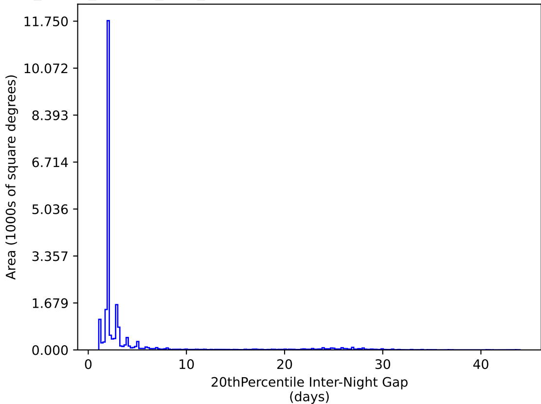
roll_pause_mjdp60_v3.4_10yrs All sky y band: 20thPercentile Inter-Night Gap
