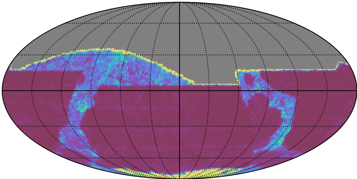
roll_pause_mjdp60_v3.4_10yrs All sky i band: 20thPercentile Inter-Night Gap
