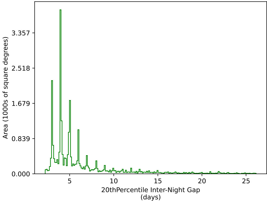
roll_pause_mjdp60_v3.4_10yrs All sky g band: 20thPercentile Inter-Night Gap
