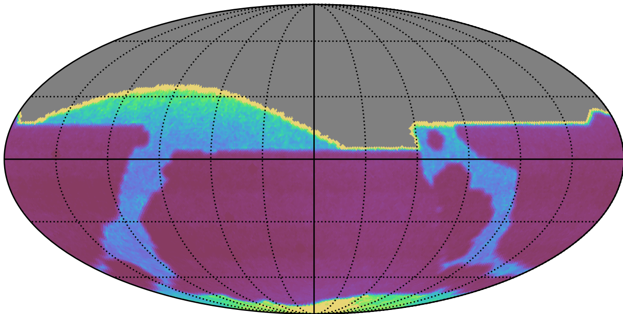
roll_pause_mjdp60_v3.4_10yrs : properMotion
