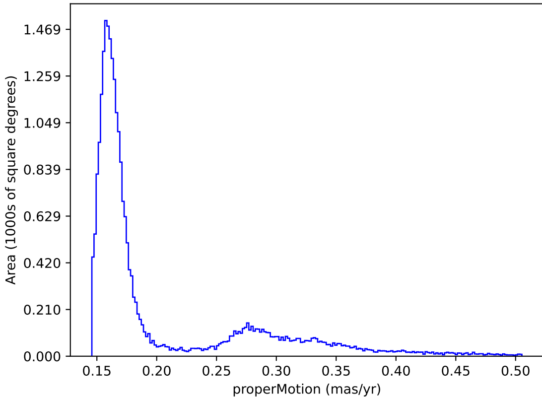
roll_pause_mjdp60_v3.4_10yrs : properMotion
