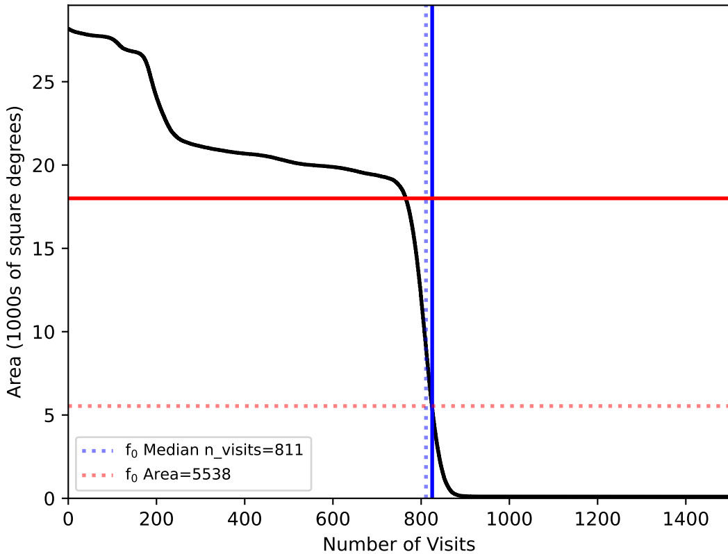
roll_pause_mjdp60_v3.4_10yrs : fO
