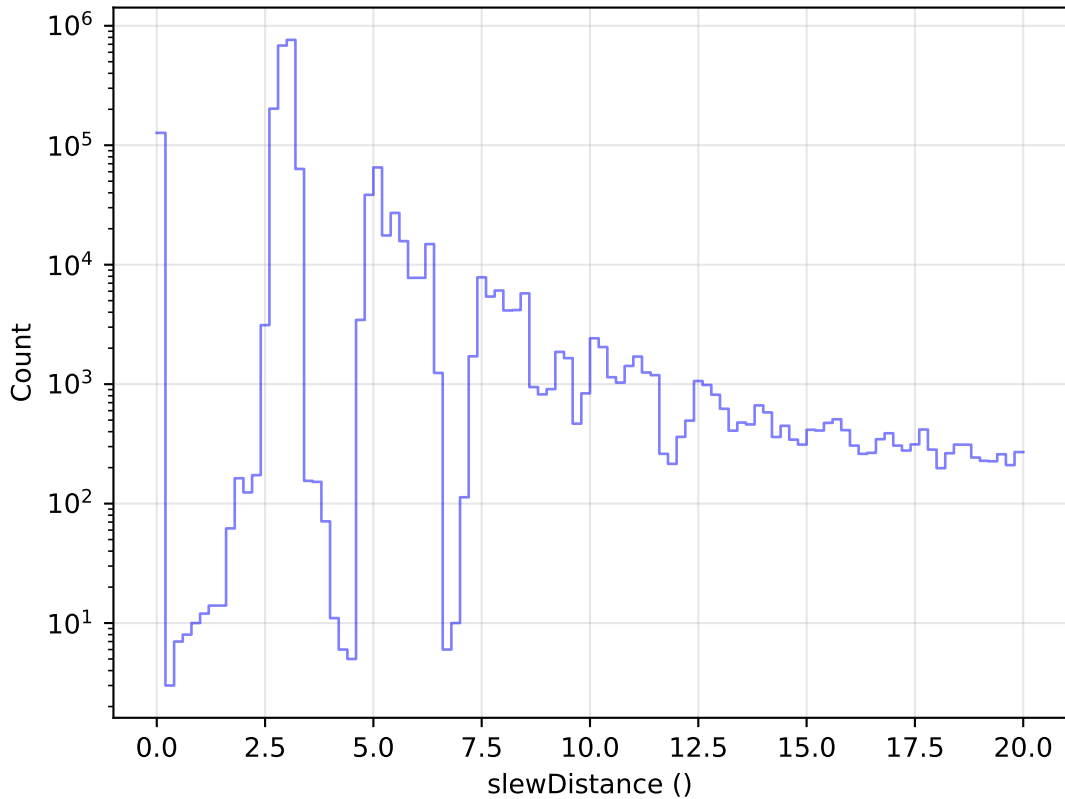
roll_pause_mjdp60_v3.4_10yrs All visits: Zoom Slew Distance Histogram
