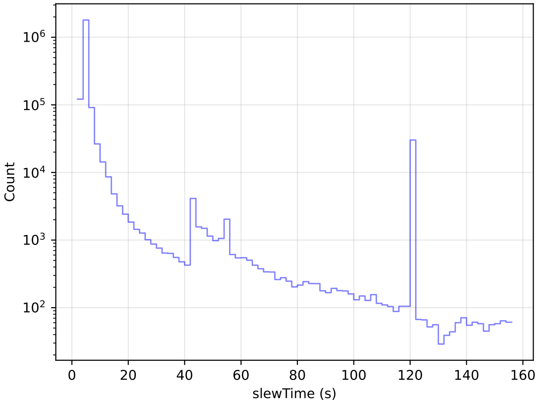
roll_pause_mjdp60_v3.4_10yrs All visits: Slew Time Histogram
