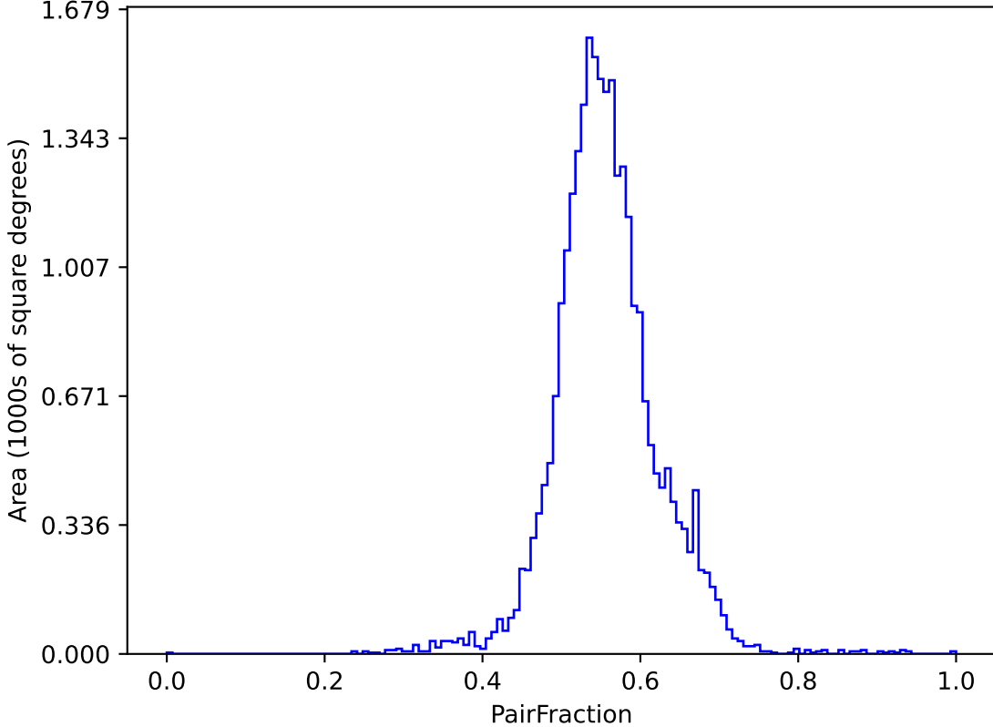
roll_pause_mjdp60_v3.4_10yrs (g or r or i): PairFraction
