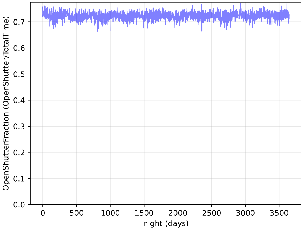
roll_pause_mjdp60_v3.4_10yrs : OpenShutterFraction
