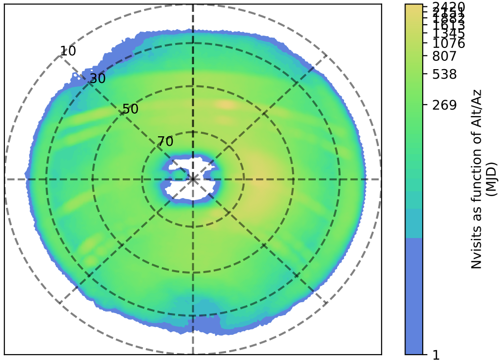
roll_pause_mjdp60_v3.4_10yrs z: Nvisits as function of Alt/Az
