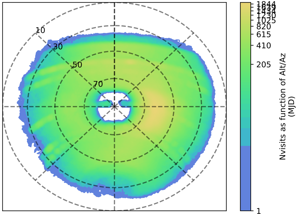
roll_pause_mjdp60_v3.4_10yrs y: Nvisits as function of Alt/Az
