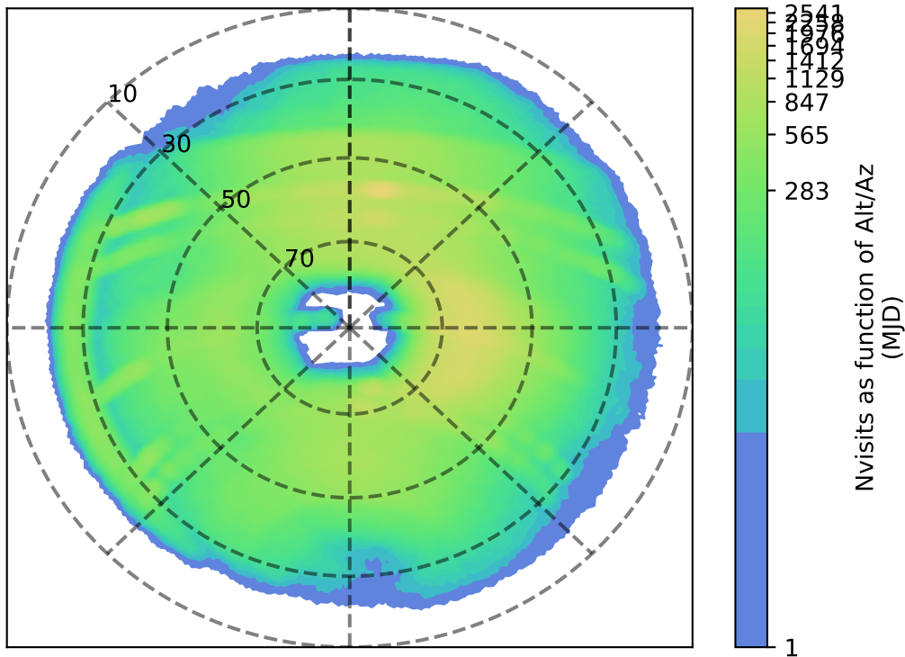
roll_pause_mjdp60_v3.4_10yrs r: Nvisits as function of Alt/Az
