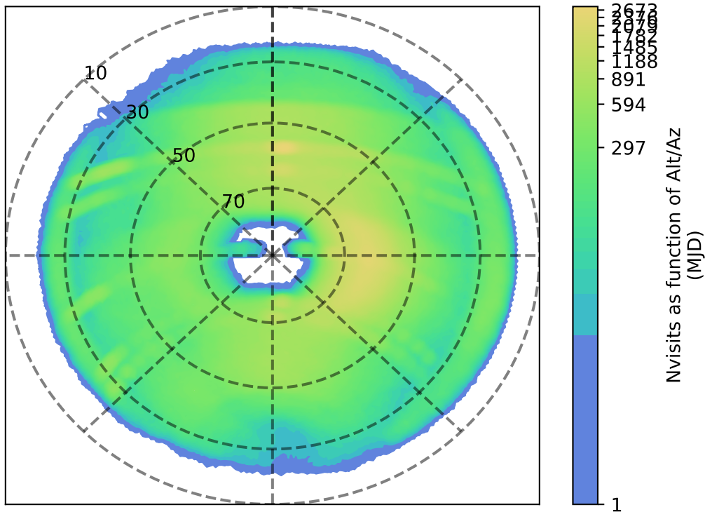
roll_pause_mjdp60_v3.4_10yrs i: Nvisits as function of Alt/Az
