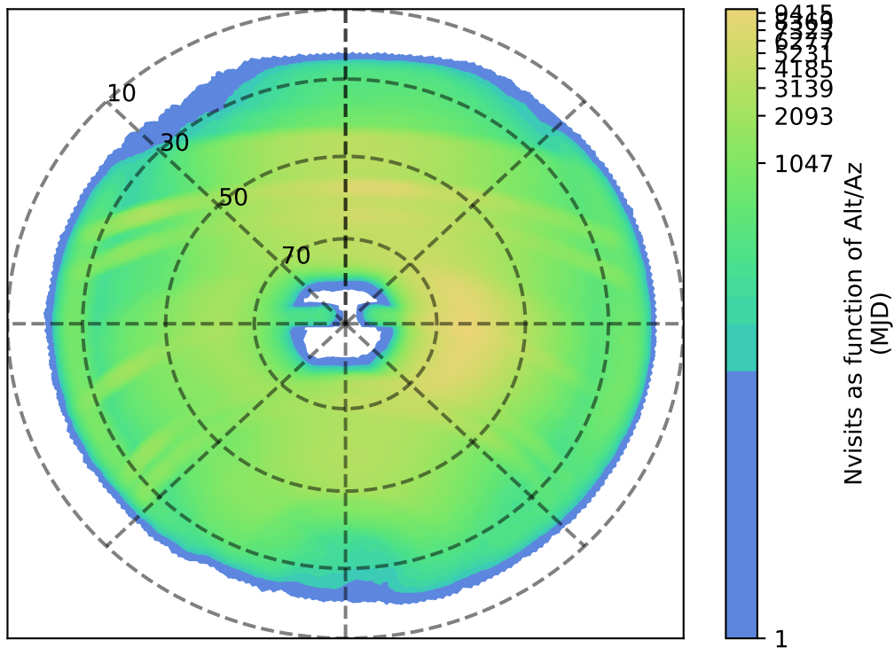
roll_pause_mjdp60_v3.4_10yrs : Nvisits as function of Alt/Az
