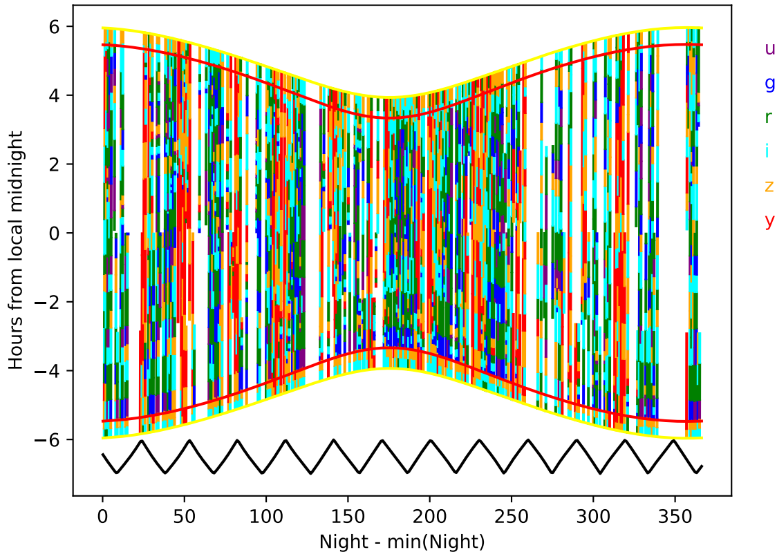
roll_pause_mjdp60_v3.4_10yrs year 7-8: Hourglass
