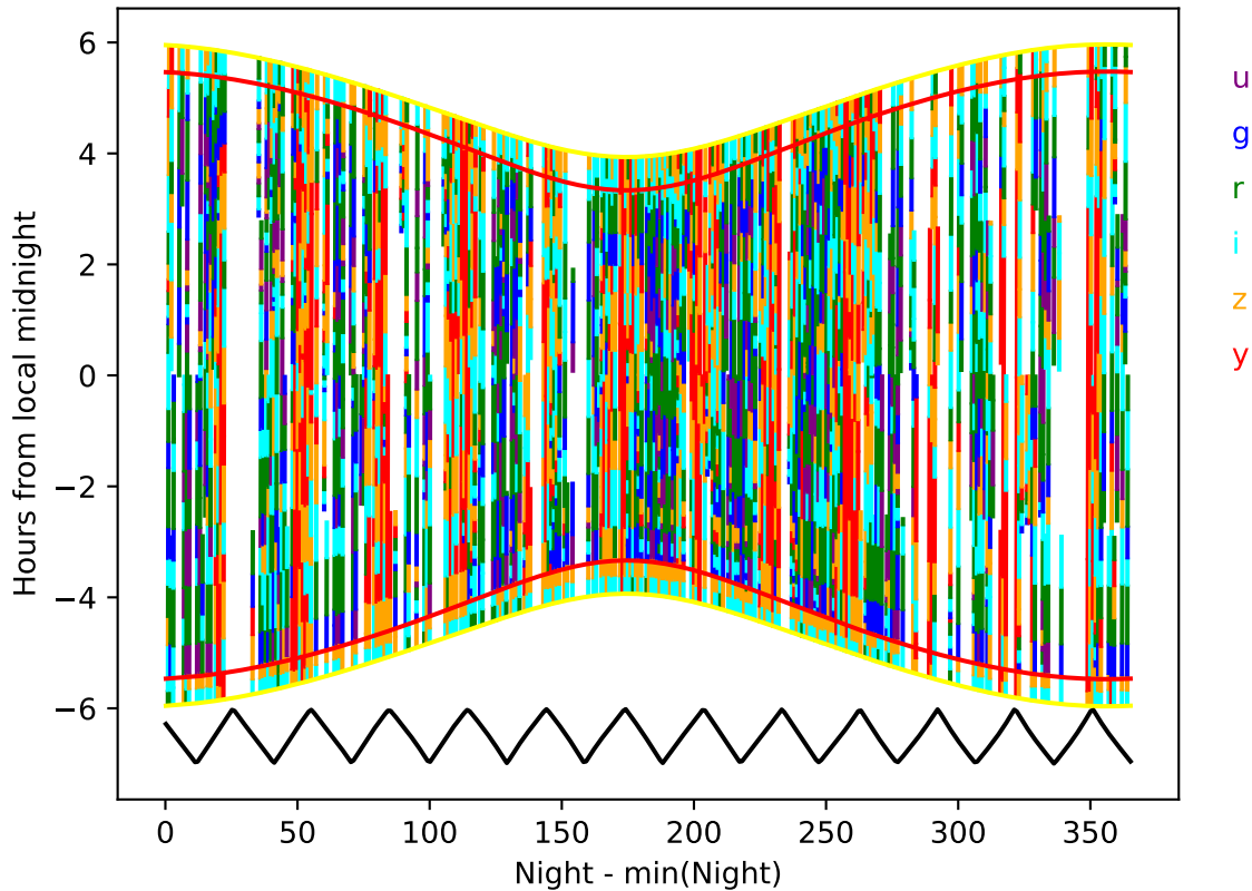
roll_pause_mjdp60_v3.4_10yrs year 4-5: Hourglass
