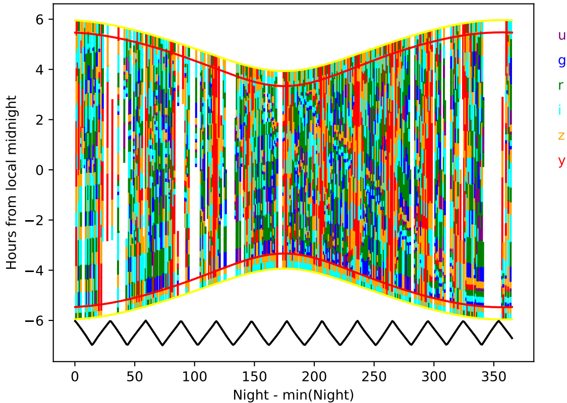
roll_pause_mjdp60_v3.4_10yrs year 1-2: Hourglass
