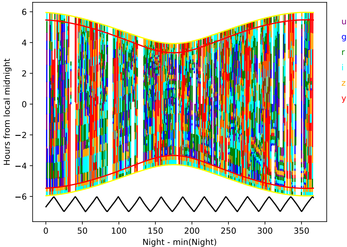
roll_pause_mjdp60_v3.4_10yrs year 0-1: Hourglass
